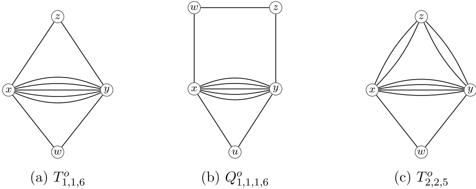
Fig. 2. The graphs T_{1,1,6}^o , Q_{1,1,1,6}^o , and T_{2,2,5}^o .
