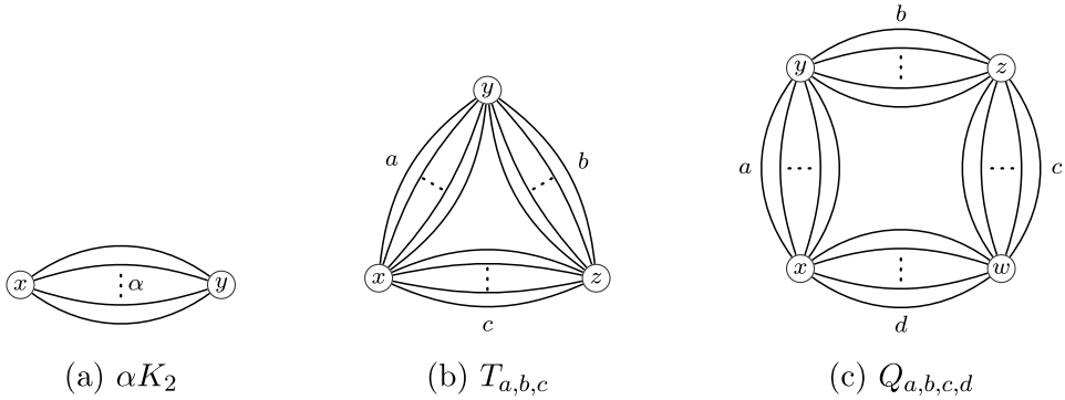
Fig. 1. The graphs \alpha K_2 , T_{a,b,c} , and Q_{a,b,c,d} .
