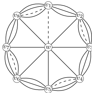
Fig. 3. The graph (\tilde{W}_8, \sigma) .
